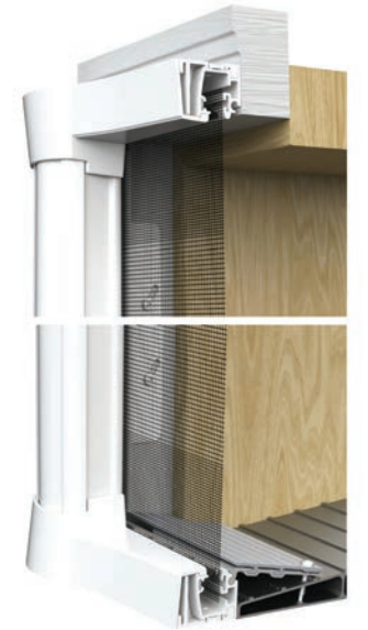
Surface / Face Mounting on a Traditional Hinged Door.
